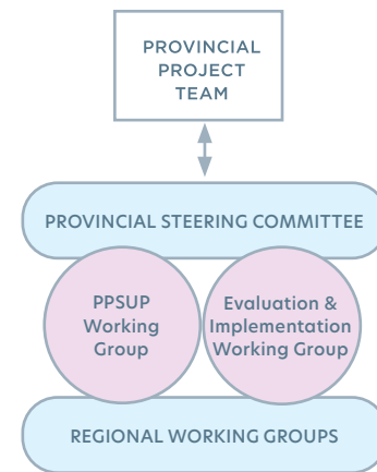
Figure 2: Project Structure
